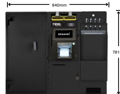
Tidel S4 with Standard Side Vault and Tube Vend
