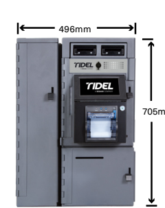
Tidel Series 4 with Narrow Side Vault
